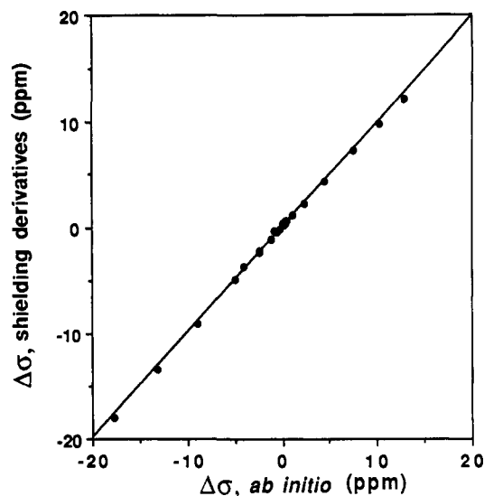
Figure 4. Additivity of structural effects on Ala C^\alpha relative shielding. The graph shows the results of varying the C^\alpha-N and C^\alpha-C^O bond lengths simultaneously using either a full ab initio treatment (horizontal axis) or by using the bond length shielding derivatives (vertical axis).
